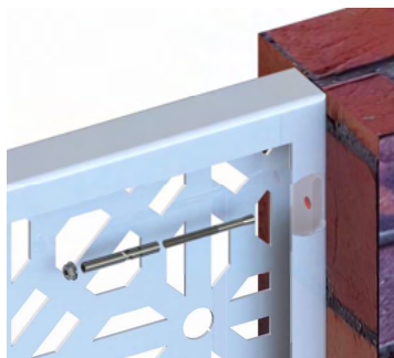
Side wall fix
