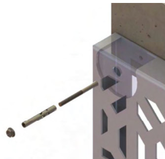
Front face fix
